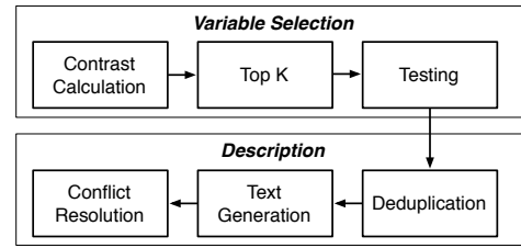
Figure 4: Workflow of Clustine’s cluster description module.
